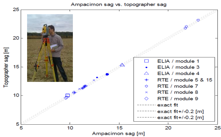
Fig. 1: Ampacimon sag measurement vs. independent sag topography measurement showed very good agreement ( \pm 20\text{cm} ).
