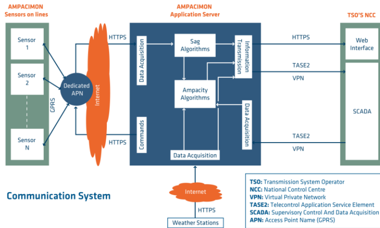
Fig. 3: IT platform developed for the Ampacimon DLR system providing real-time ampacity and short-term forecast. Those outputs are coupled with TSO's quarter-hourly network security calculation software.
