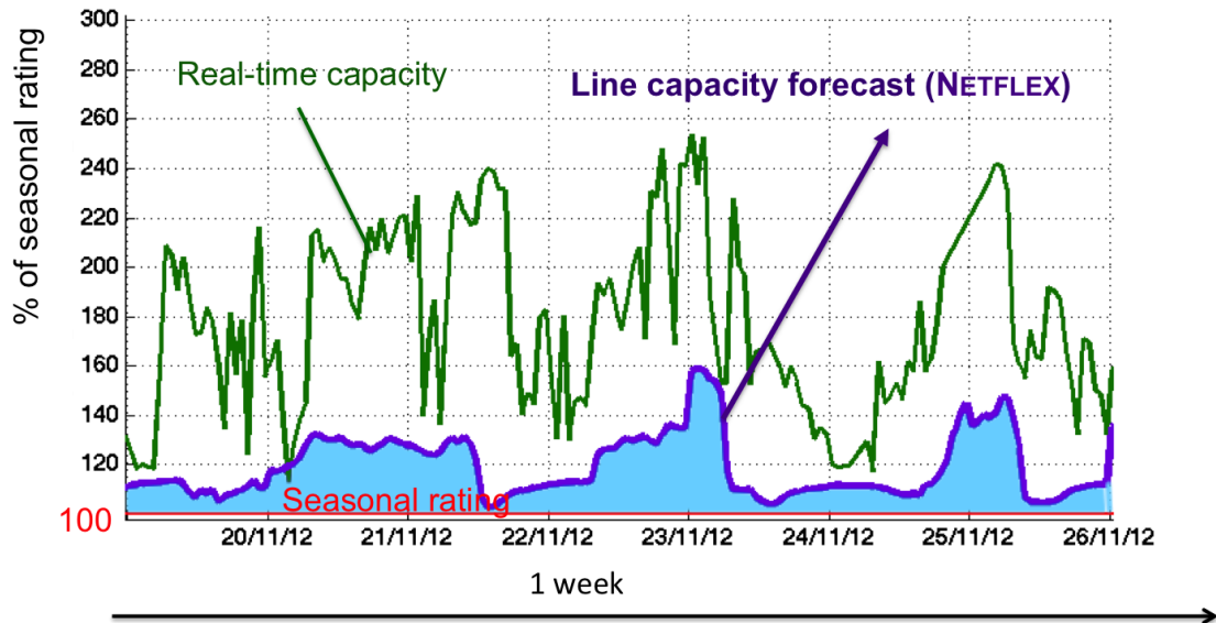
Fig. 5 : (i) real-time capacity (=ampacity) and (ii) Twentys two-day ahead forecast, developed at the University of Liège, Belgium, guarantees a safe ampacity forecast.
